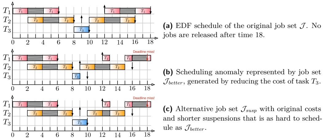
■ Figure 1 (adapted from [2]) Three schedules under the segmented suspension model showing that the impact of the lack of sustainability tightly depends on the considered task model. Despite the anomaly shown in schedule (b), there exists a harder schedule (c) with no anomaly that still incurs a deadline miss. If we assume that the task model allows variable suspension times, then any schedulability analysis that covers all possible scenarios would not claim the job set in (c) (and thus the task set) to be schedulable, regardless of the anomaly present in schedule (b).
