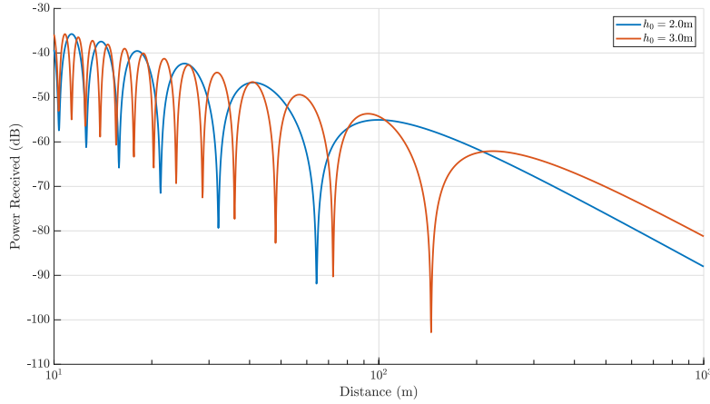
Fig. 2. Two-ray model showing that received power is affected by both the link distance and the antenna height ( h_0 ) relative to the reflective surface.
