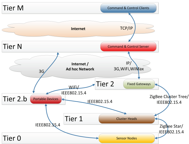
Figure 1: EMMON Hierarchical System Architecture.
