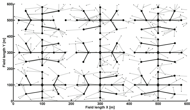
Figure 3: Example of WSN Patches with a SBD scheme to cover at least 80% of a 49 km 2 field (particular). Diamond markers are GWs; stars are CHs, distributed along 2 hops around each GW; points are SNs, randomly deployed.
