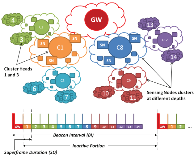
Figure 6: Time Division Cluster Scheduling (TDCS): it is assumed that every cluster has the same value of the couple (BO, SO). The inactive portion of the GW (only) is also shown, as an example.
