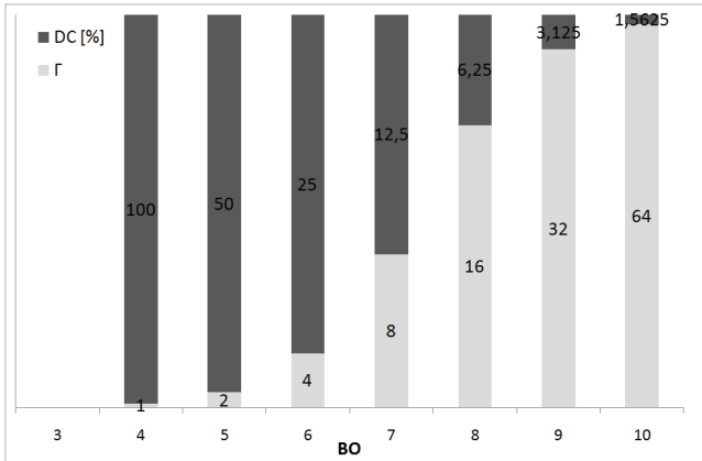
Figure 7: TDCS: upper bound on the allowed number of clusters ( \Gamma ) and related duty cycles (DC) for SO=4 and a subset of values of BO.
