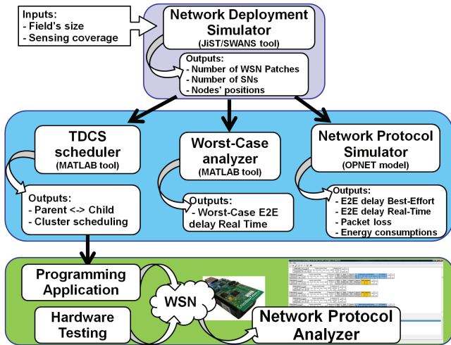
Figure 2: EM-set: EMMON toolset for network planning, dimensioning simulation analysis and test/programming.
