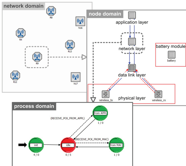
Figure 9: The structure of the IEEE 802.15.4/ZigBee Opet simulation model.
