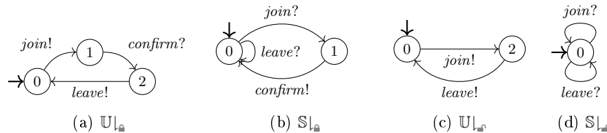
Fig. 2: Product models of users and servers (projections of the models in Fig. 1)
